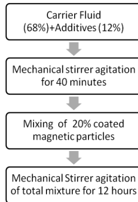
FIGURE 2. Structural outline for preparation ofMR Fluid
