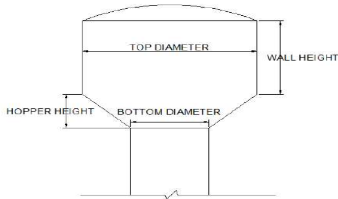
Fig. 1 General Diagram of Intze Water tank
