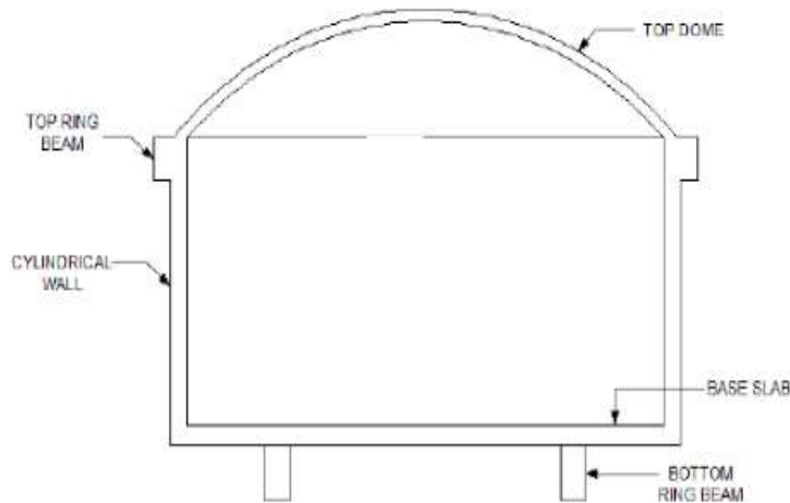
Fig. 2 General Diagram of Circular Water tank
