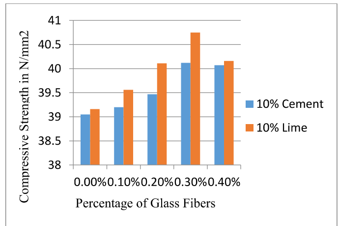
Graph 4 Rebound Hammer Compressive strength of Glass fiber Geopolymer Concrete after 28 days With cement and lime.
