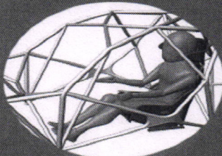
ROLL CAGE DESIGN
