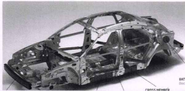
Body In White (BIW)
